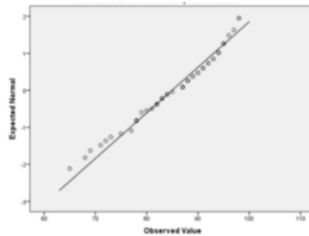
Normal Q-Q plot of English skills
