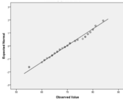
Normal Q-Q plot of YouMiMe
